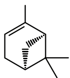
(-)- \alpha -pineno
